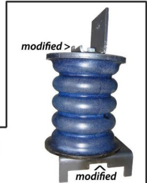
modified > Front Driver's Side SumoSprings SSF-181 Uninstalled
